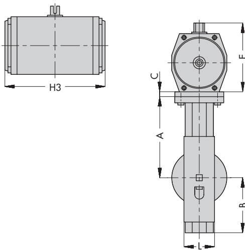
Type 3335/31a Butterfly Valve
